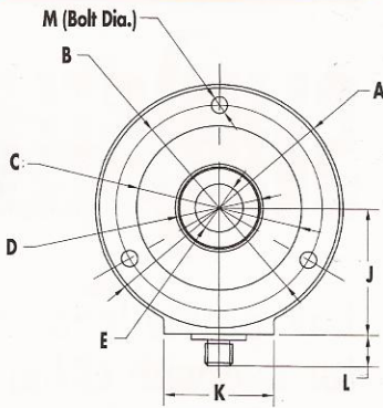
Slim Cell (alone)
